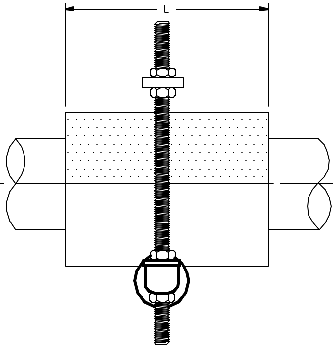
ELEVATION VIEW
