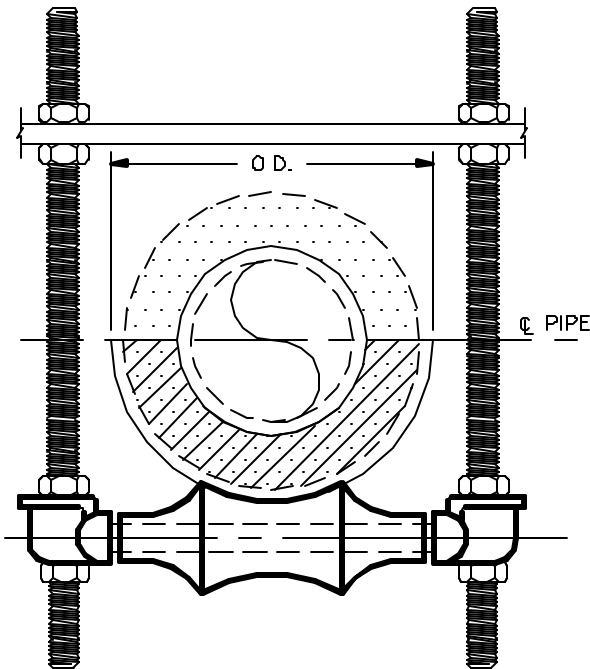
END VIEW
