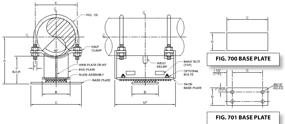
FIG. 700 - WELDED BASE
