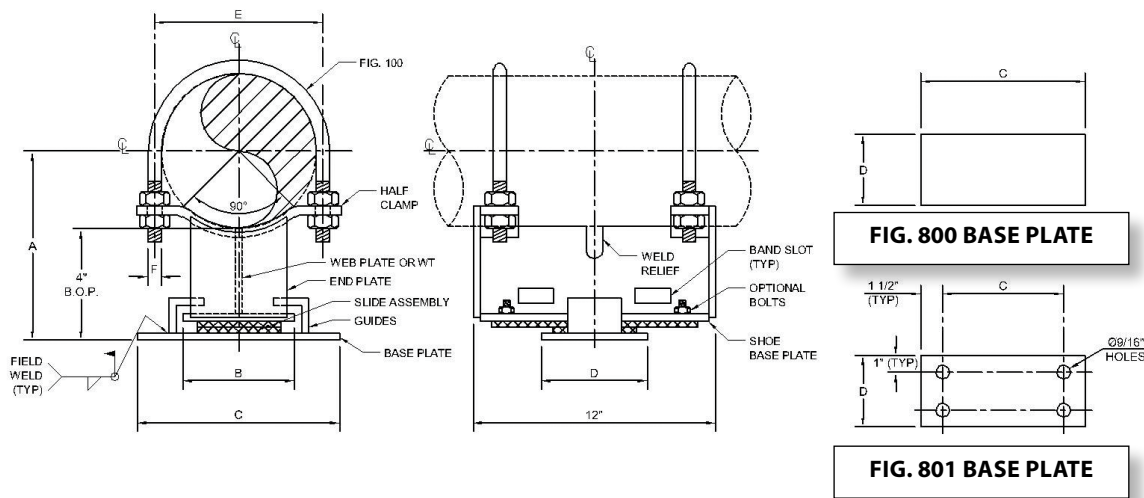
FIG. 800 - WELDED BASE
